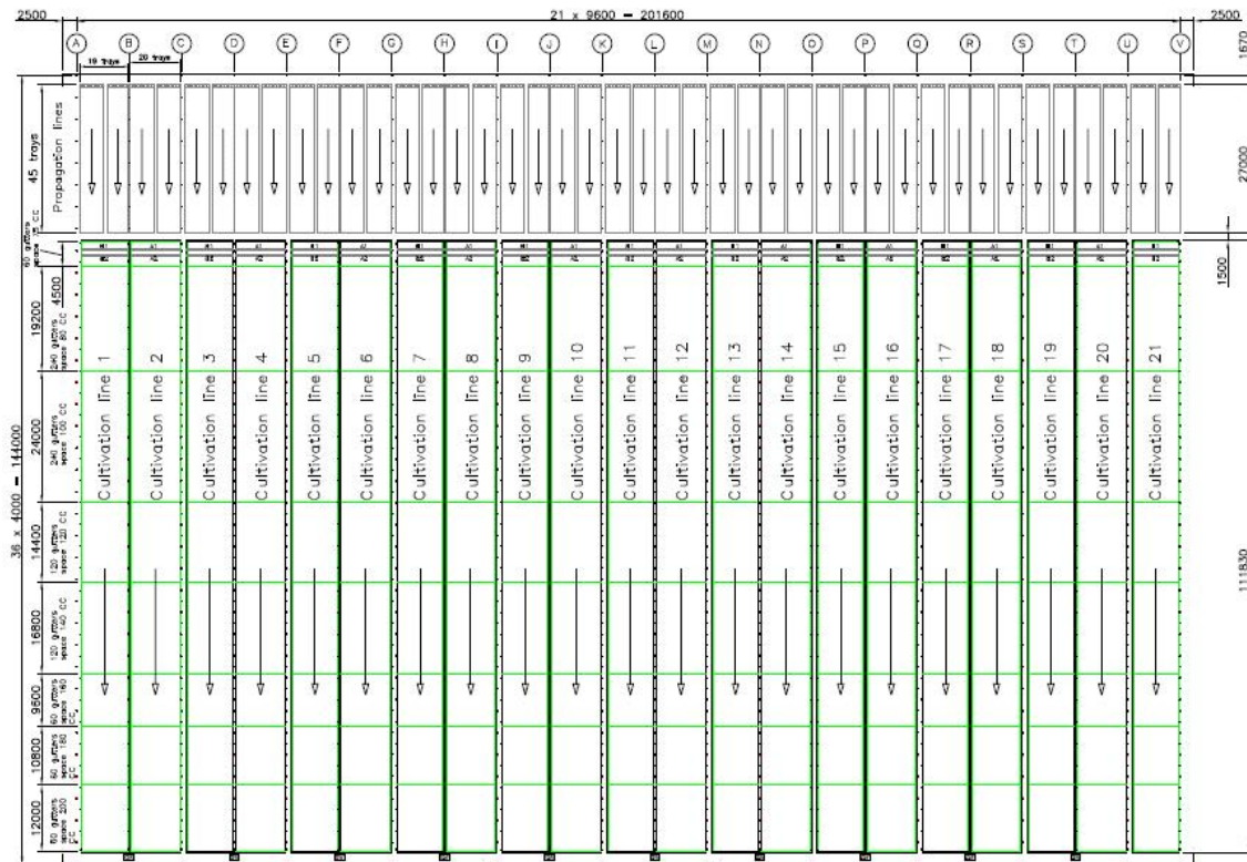
Example of greenhouse with propagation area and gutter lines.
